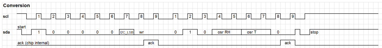
Figure 5 Conversion Command
