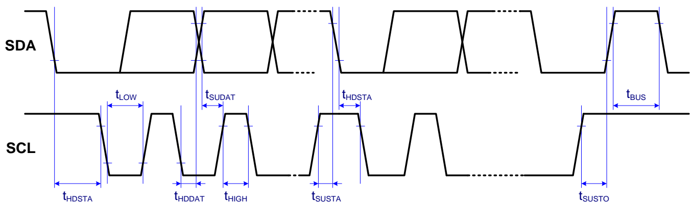
Figure 15. Bus Timing
