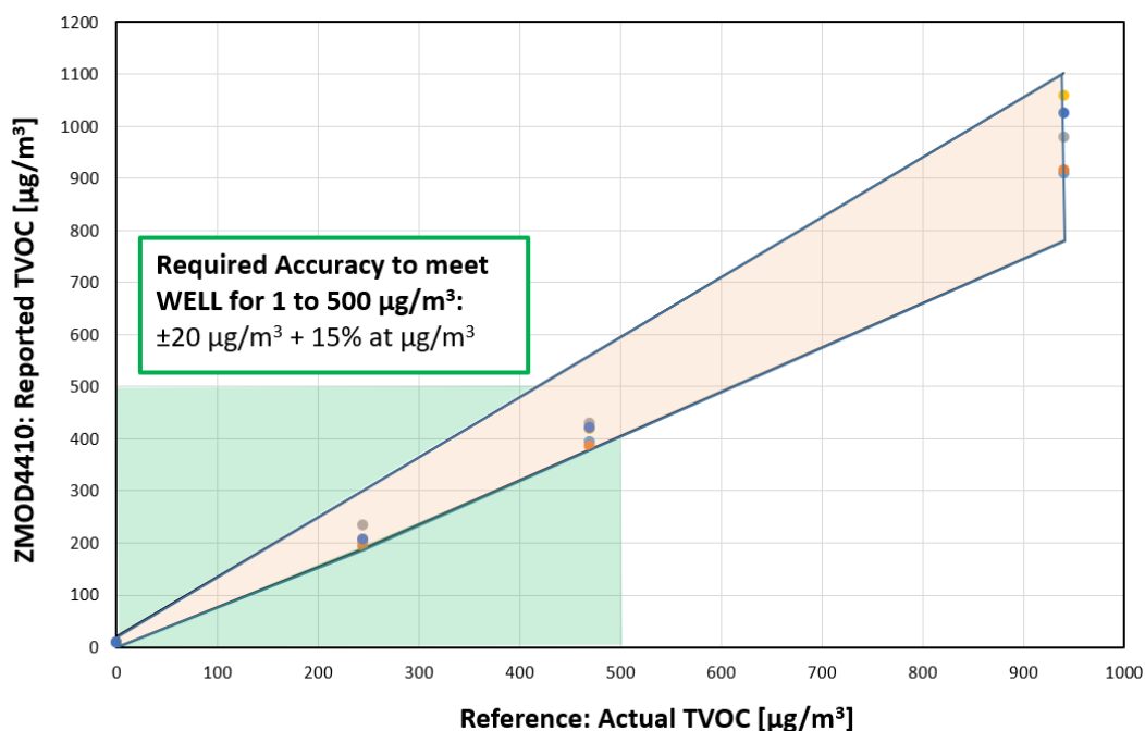
Figure 8. TVOC Measurement according to WELL Standard using ZMOD4410
