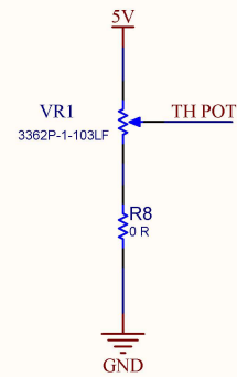
THRESHOLD POT
