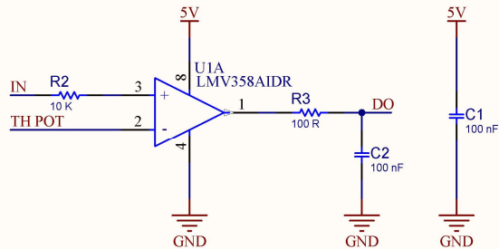
COMPARATOR CIRCUIT
